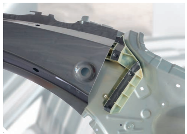
Reinforcer application examples 1 B-pillar junction with roof frame 2 C-pillar application
