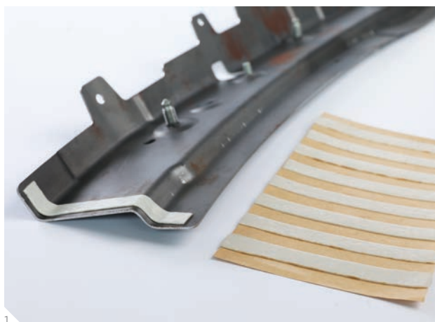
1 C-pillar junction with frame with extruded reinforcer tape
