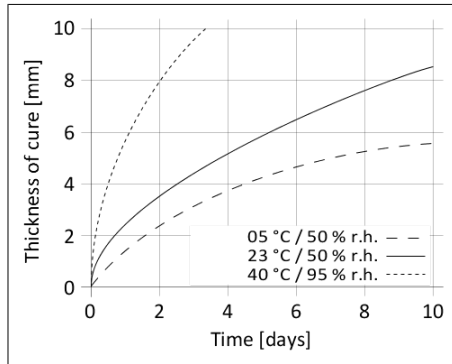
Diagram 1: Curing speed Sikasil® WS-305 S
