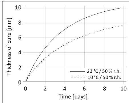
Diagram 1: Curing speed of Sikaflex®-515
