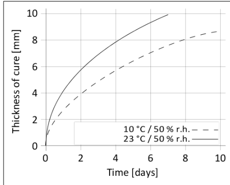
Diagram 1: Curing speed Sikaflex® SOLO
