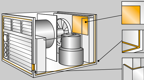
Metal frame sealed and bonded with Sikaflex®-268 . For primer-free applications, Sikasil® AS-70 or the fast cure Sikasil® AS-785 are advised.
